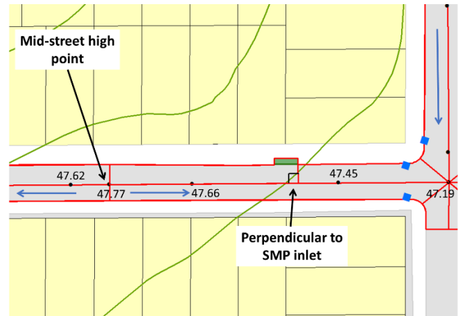
Figure 6.4. Example boundaries at inlets of PC SMPs.
