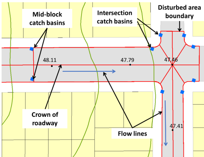
Figure 6.2. Example delineation of disturbed drainage areas with separation lines for the crown of roadway and catch basins.
