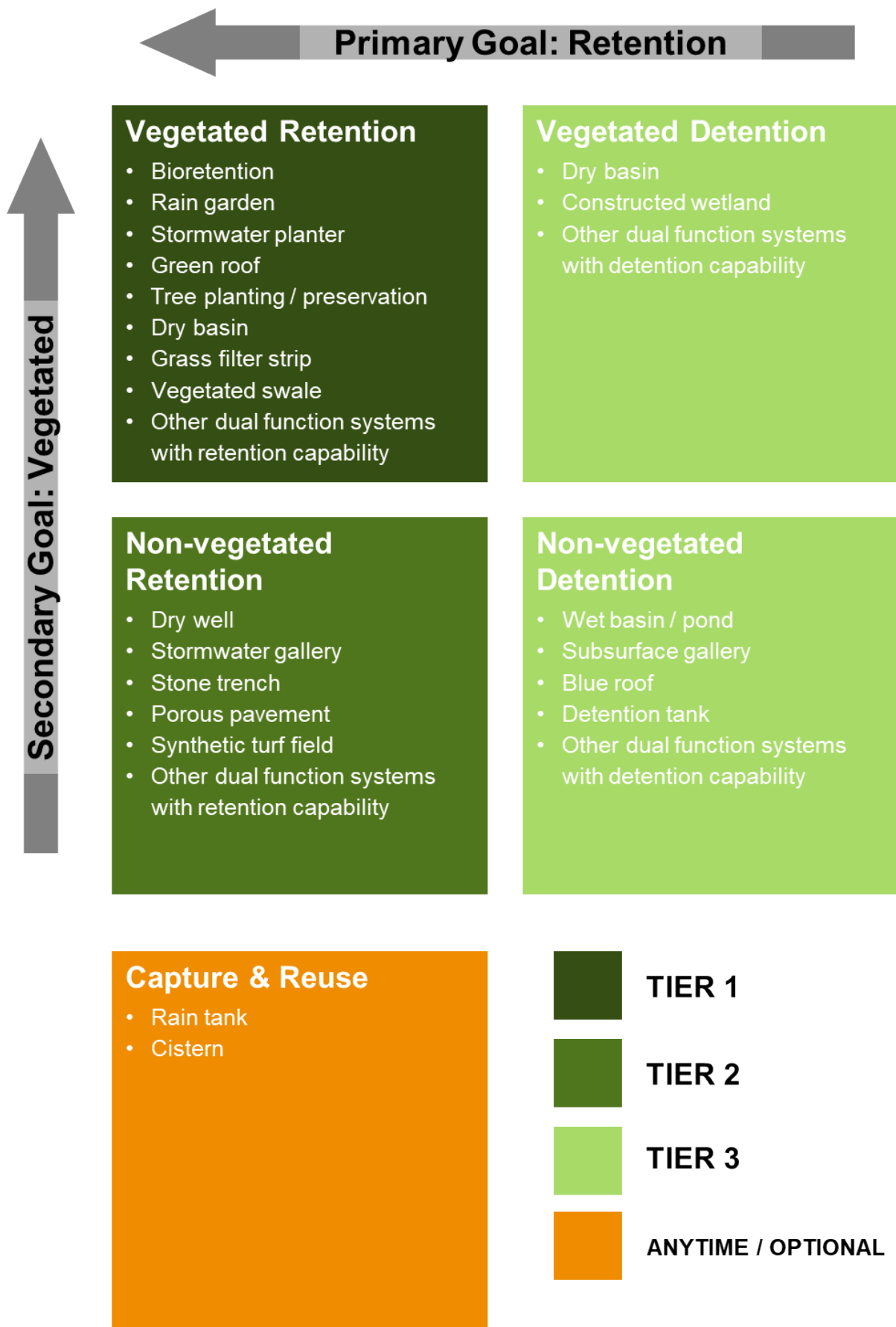
Figure 4.2. SMP hierarchy for CSS areas.
