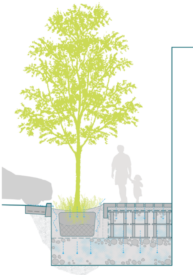
Figure 4.5. Illustration of a hybrid system that incorporates bioretention and porous pavement features (image courtesy of SCAPE).
