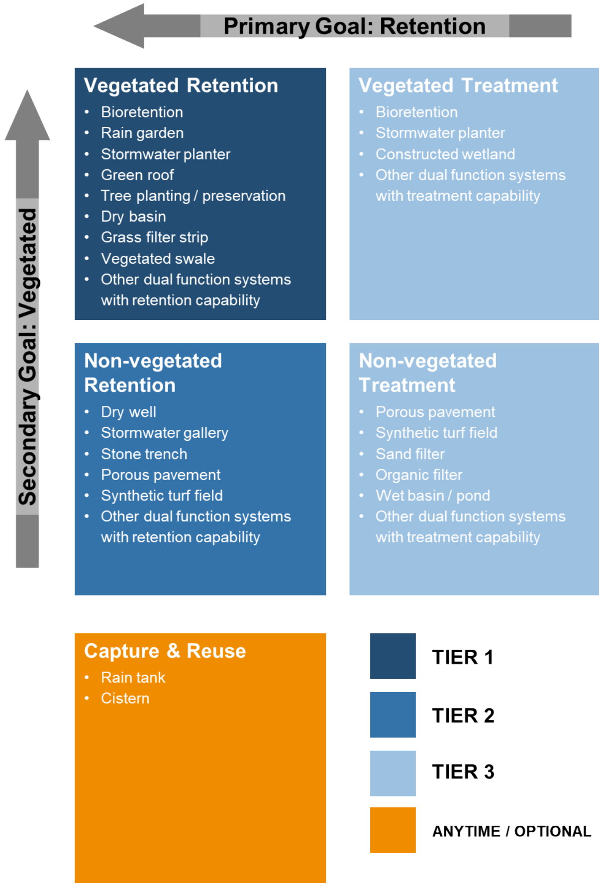
Figure 4.3. SMP hierarchy for MS4 areas.
