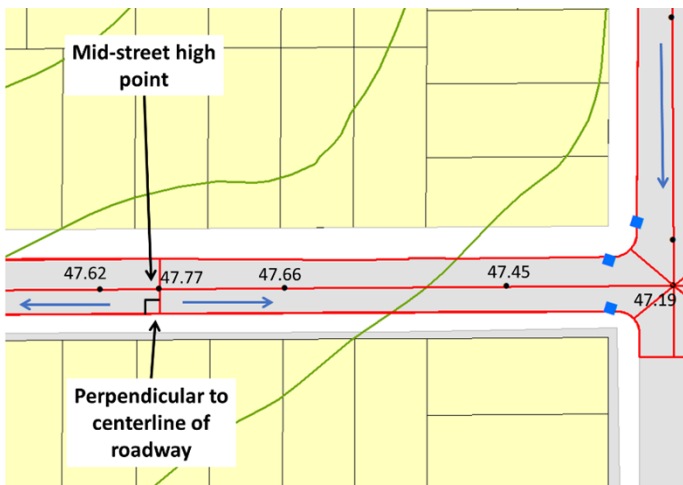
Figure 6.3. Example delineation of disturbed drainage areas with added separation lines at high points.
