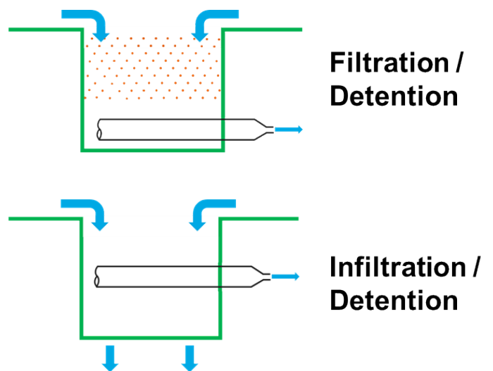
Figure 4.6. Illustration of the two most common dual function systems.
